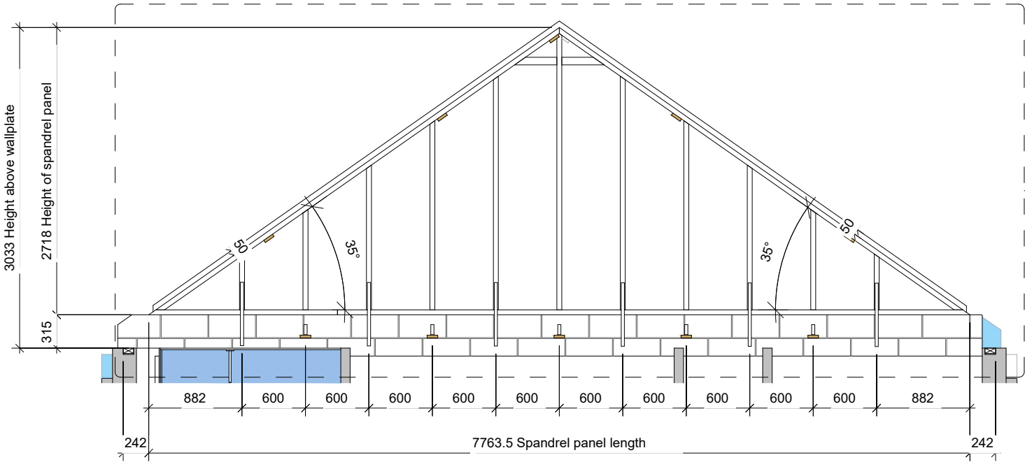
T2 Spandrel Panel - 1no reqd (1ply, 470kg) 1 : 50
