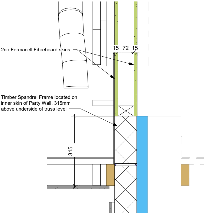
T3 Spandrel Panel - Section Through Base 1 : 10
